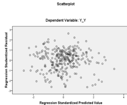
Gambar 1. Scatterplot
